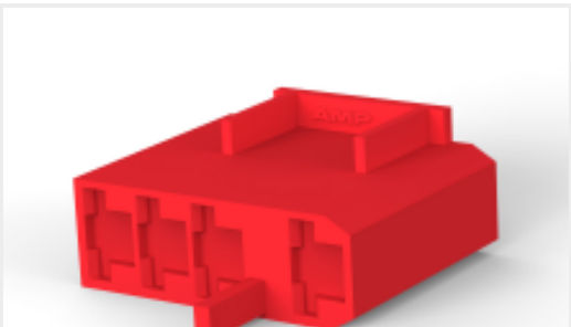
TE Part #2-521498-2 250 FASTON HSG.,REC.,4 POS,RED
