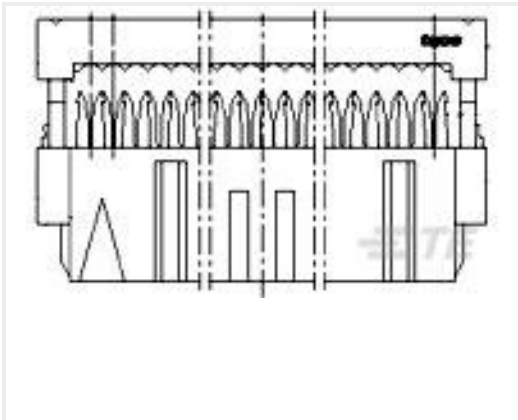
TE Part #2-215882-0 20 WAY GREY MK II RECP
