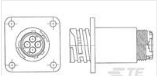
TE Part #788154-2 SLD CPC RCPT ASSY,11-4,REV SEX
