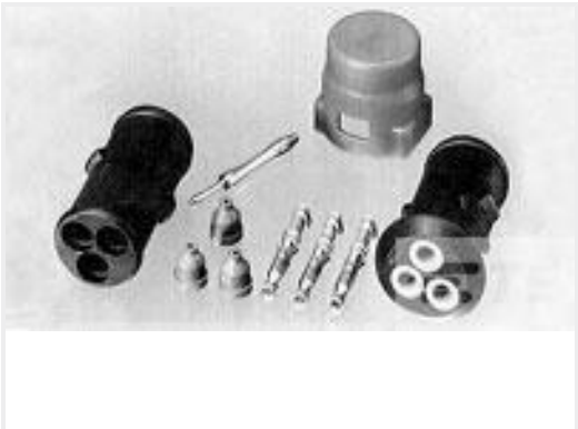
TE Part #1-826886-2 3N ECONOSEAL HYLSYR
