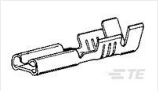
TE Part #140717-1 110 FASTON,REC.,22-18 AWG,BR
