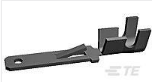
TE Part #180352-2 FF 250 TAB 4-6MM2 PTBR
