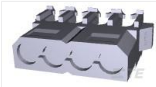
TE Part #1735539-2 Slimline SATA Receptacle, Vertical, SMT
