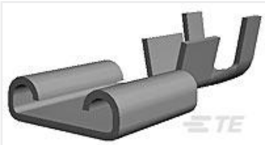
TE Part #170224-2 250 FASTON,REC.,16-10 AWG,BR
