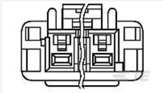
TE Part #2-1376388-3 5MM POWER KEY 2P PLUG HSG BLUE
