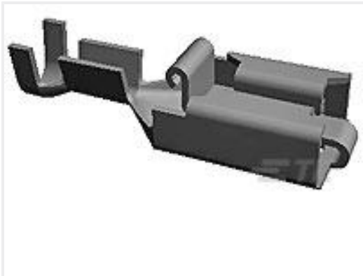
TE Part #341001-3 PL 250 REC TERMINAL 13-11 TPBR LP
