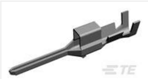
TE Part #917765-1 2.5 SIGNAL D/LOCK TAB CONT. M
