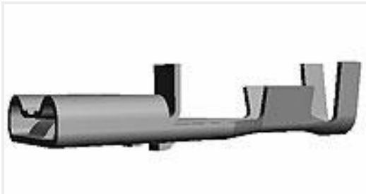
TE Part #170328-1 250 PL MKII REC. 18-14AWG PTBR
