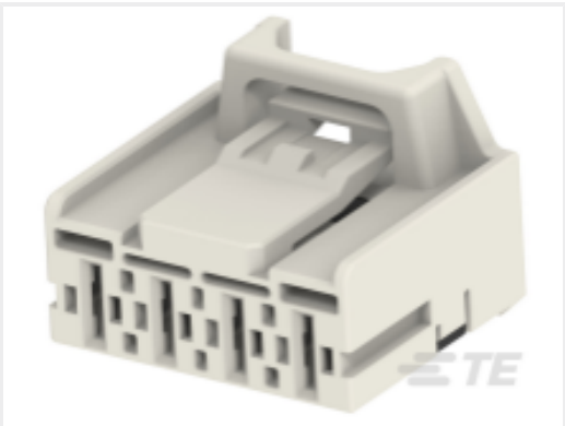
TE Part #2299956-1 MCP 6.3MM 4P PLUG ASSY A
