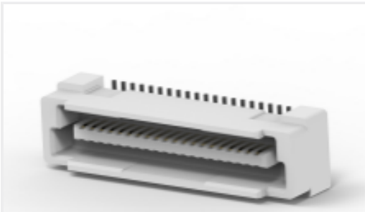
TE Part #CAT-313-PCB40 Free Height Plug Connector: Board-Board, Vertical, 40, 0.8mm
