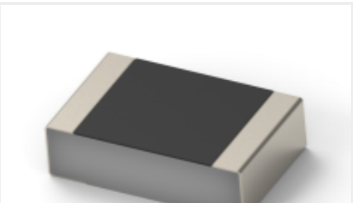
TE Part #7-2176453-7 CPF 0201 35K7 0.1% 25ppm 1K RL
