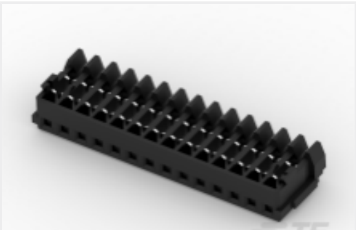
TE Part #3-353293-4 1.5MM CT MT REC ASSY 14P BLACK
