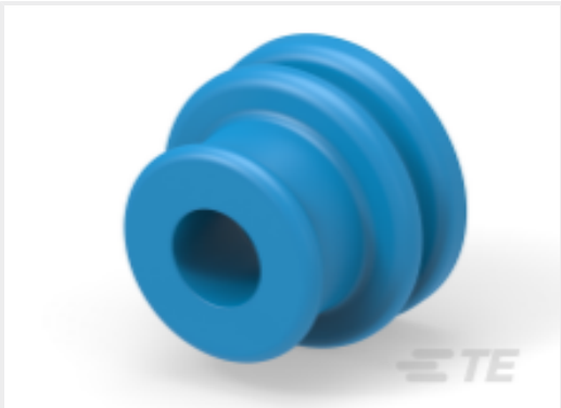
TE Part #2391530-2 SINGLE WIRE SEAL, 1.95-2.50
