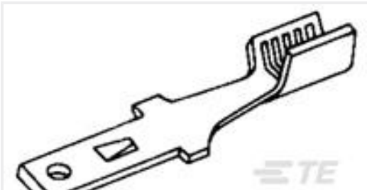
TE Part #62445-1 187 AMVAR FFTAB FLT 020TPBR
