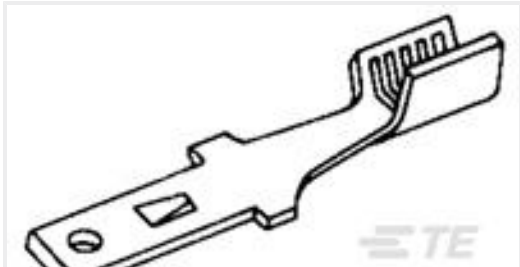
TE Part #62447-1 187 AMVAR FFTABFLT 020TPBR
