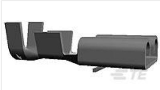
TE Part #42281-1 FF 250 REC 18-14AWG BR
