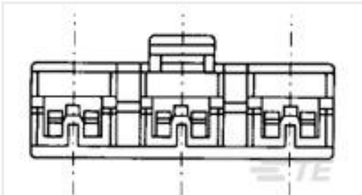
TE Part #353255-7 110 HSG. PL EX REC. 7.6mm 3P RED
