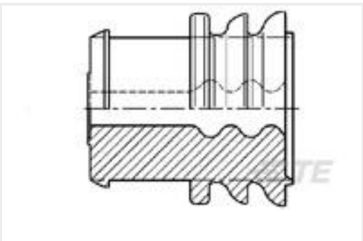
TE Part #100132-1 CAVITY PLUG
