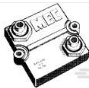
TE Part #1614770-4 BDS 2 A 250 10R 10%
