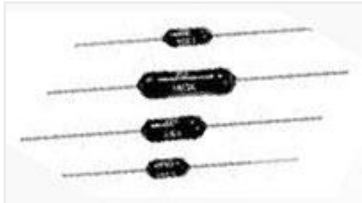
TE Part #4-1879627-8 H4P 910R 1% 100PPM
