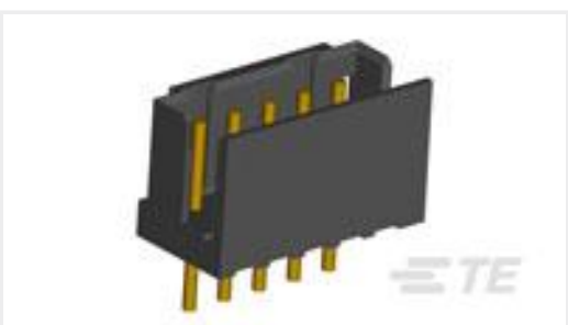
TE Part # CAT-3984552-PHITPS CT Post Header Assembly: Part. Shrouded
