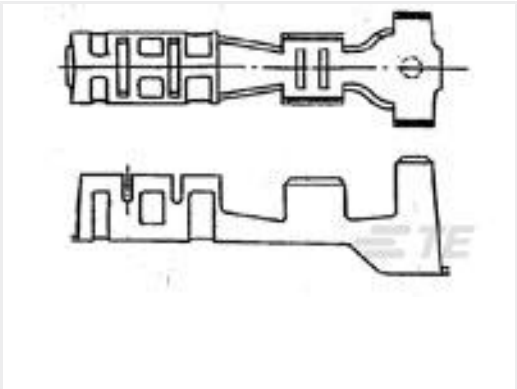
TE Part #175135-1 CONTACT 22-18 AWG 0.30 X 17.0 PTKLF-5
