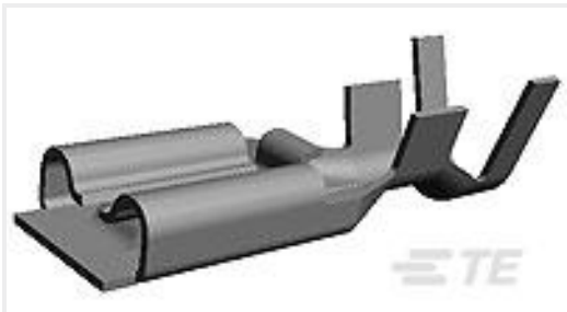
TE Part #175032-1 PL 187 REC 26-20 AWG 0.30 X 14.0 SS
