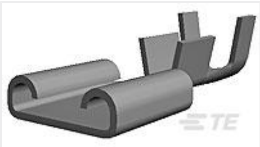
TE Part #735209-2 250 FASTON REC 22-18 AWG TPBR
