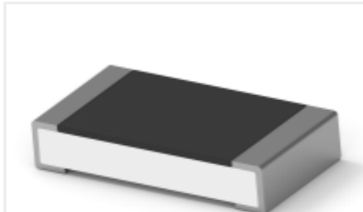
TE Part #9-2176391-7 RQ 1206 124K 0.1% 10PPM 5K RL
