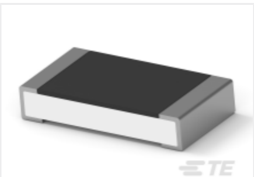
TE Part #9-2176391-6 RQ 1206 121K 0.1% 10PPM 5K RL
