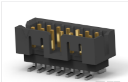
TE Part #1-2842246-4 14P,2MM,SHRD HDR,DRV,T,SMD,0.76 AU,TB W/CP
