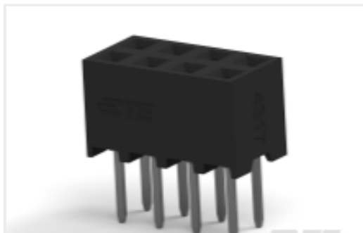
TE Part #2314820-8 8P,2MM,B-B,REC,DRV,T,2,7,0.1AU,TB
