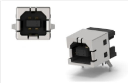
USB Type B Connectors(1)
