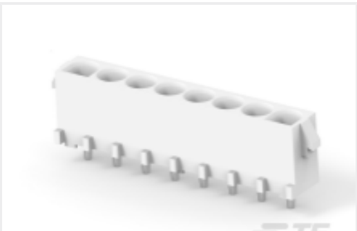
TE Part #826844-7 UMNL PC PIN HEADER 8POS
