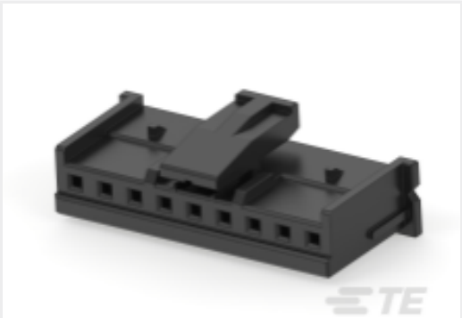
TE Part #4-2338183-9 EP 2.5 HOUSING 9P, BLACK, UL version
