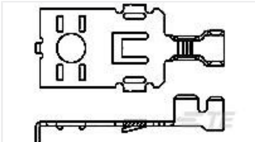
TE Part #63166-4 POWER RING,TERMINAL 16-12 AWG BR
