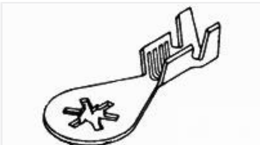
TE Part #62613-2 RING .190 12-10 AWG 0245 TPCRS
