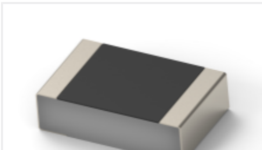
TE Part #6-2176453-6 CPF 0201 27K4 0.1% 25ppm 1K RL
