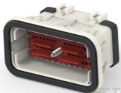
TE Part #1599185-2 HSG ASSY 76 POS PIN CONTACT
