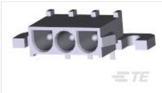
TE Part #3-350943-0 03P UMNL HDR ASSY R/A 94VO LF
