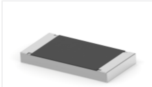
TE Part #2176350-5 CRGCQ 2512 4R7 5%
