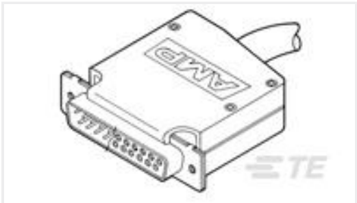
TE Part #5206393-1 AMPLIMITE ASSY, SIZE 2
