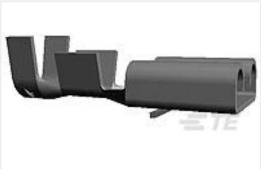
TE Part #5-160446-5 FF 250 REC 1.0-2.5MM2 TBPR
