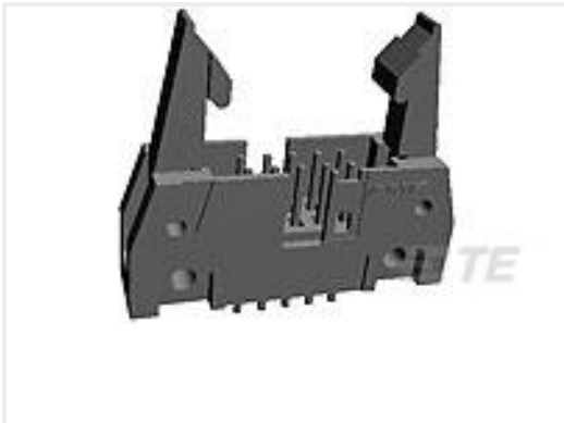
TE Part #5499160-6 A/L UNIV HDR 26P VERT SHT LAT
