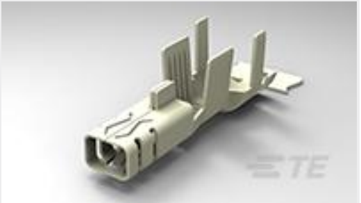
TE Part #1971781-1 PTL RECEPTACLE CONTACT, 14 AWG
