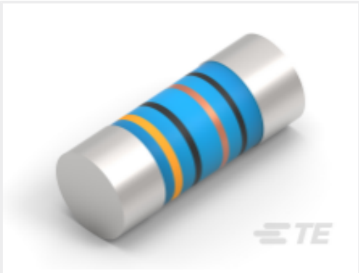
TE Part #8-2176315-0 MELF SMA-A 27R 1% 50PPM 0204 0.4 W
