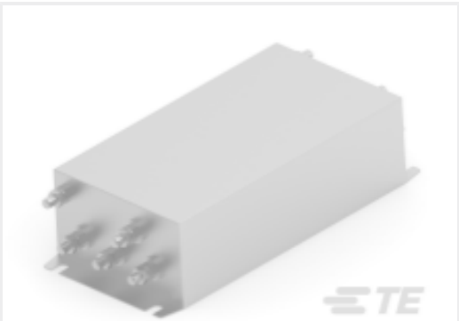
TE Part #2-1609968-4 KEP 150A 1S HIGH PLUS NUT WYE 440VAC
