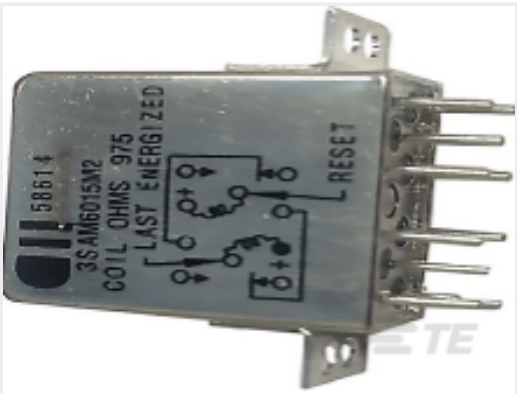
TE Part # 3-1617522-6 3SAT1302A2=M5757/13-085
