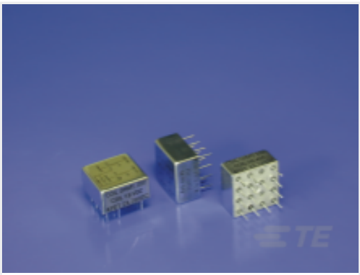
TE Part # CAT-3SBH-4PDT-WOCS 4PDT Signal Relay: Electrically-Held, 1 /5-Size Relay
