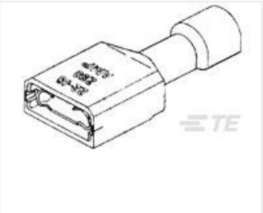
TE Part #2-520979-2 ULTRA-FAST .110/.125 ASY REC 22-18 TPBR
