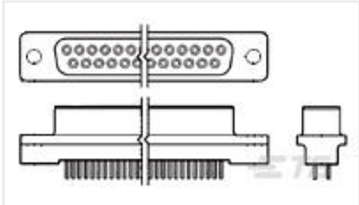
TE Part #207826-3 09 RCPT SP/AP STD
