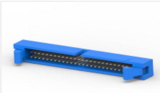
TE Part # 1-1761685-5 IDC LOW PRO HDR 50P VERT SHT LAT
