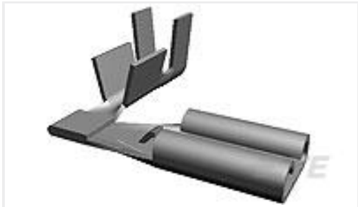
TE Part #62336-2 110 FASTON FLAG REC 22-18 AWG NPST
