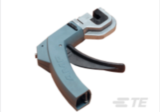
TE Part # 58372-1 HEAD (IDC) 2MM C.T. W/O TL
