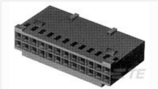
TE Part #3-87631-0 34 MODIV HSG DR MRKD .100 POL
