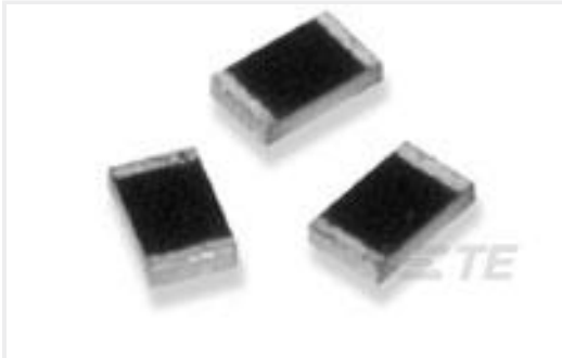
TE Part #6-1879746-3 RP 1J 26K1 0.1% 15PPM CUT LENGTH
