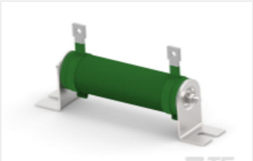
TE Part #5-1879441-5 TE 50W 2K7 5% Bracket
